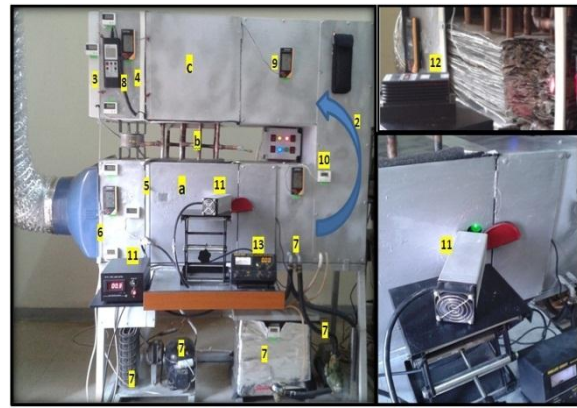
Fig (2): complete test rig of thermosyphon heat pipe heat exchanger. 1. Heat pipe heat exchanger (HPHE)a. Evaporator section b. Adiabatic section, c. Condenser section,2. U Duct,3. Fixed variable speed Fan,4. Rotated plate,5. Air filter,6. Air heater,7. Chilled water coil system(CWC),8.Digital anemometer,9.Terminator, 10.Thermometer, 11. Diode laser with wavelength 532nm, 3W power,12 .Diode laser with wavelength 650nm, 0.13W power, 13.Detector .
